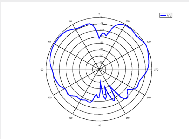
5G-1 (PHI=90) (2.4G-to-5G switchover )
