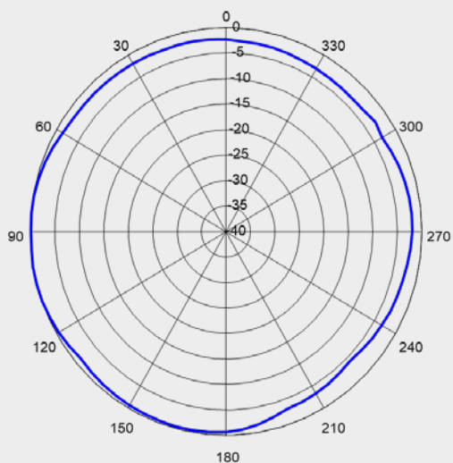
2.4G (PHI=0)
